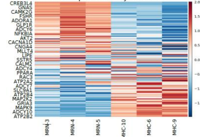
cAMP signaling pathway Homo sapiens hsa04024 Heatmap of the Analyzed Geneset
