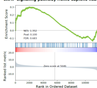
cAMP signaling pathway Homo sapiens hsa04024
