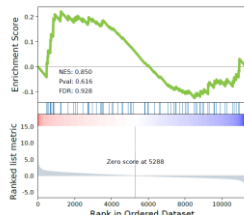
Natural killer cell mediated cytotoxicity Homo sapiens hsa04650
