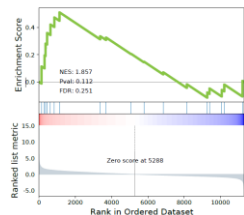
Drug metabolism - other enzymes Homo sapiens hsa00983
