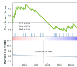
Cytosolic DNA-sensing pathway Homo sapiens hsa04623
