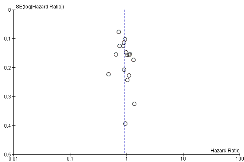
Suppl 6: (B)- Overall Survival (OS) sensitivity analysis funnel plot
