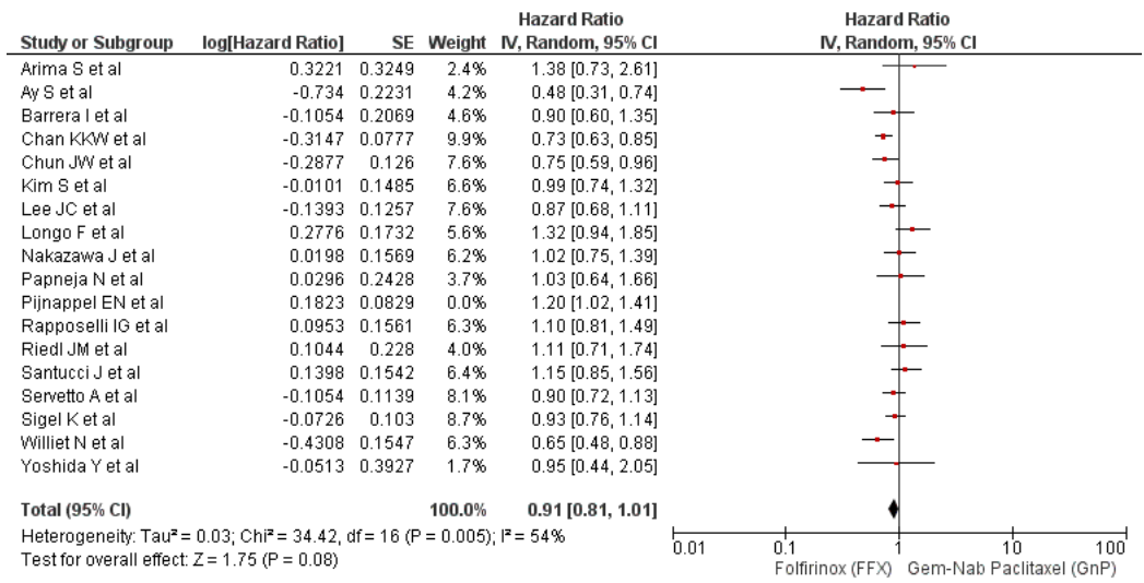
Suppl 6: (A)- Overall Survival (OS) sensitivity analysis forest plot (HR 0.91, 95% CI 0.81- 1.01; p=0.005).
